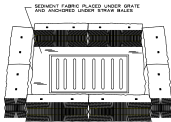
STRAW BALE BARRIER
